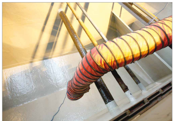
Effluent resistant DAF cell tank for a food preparation factory.
