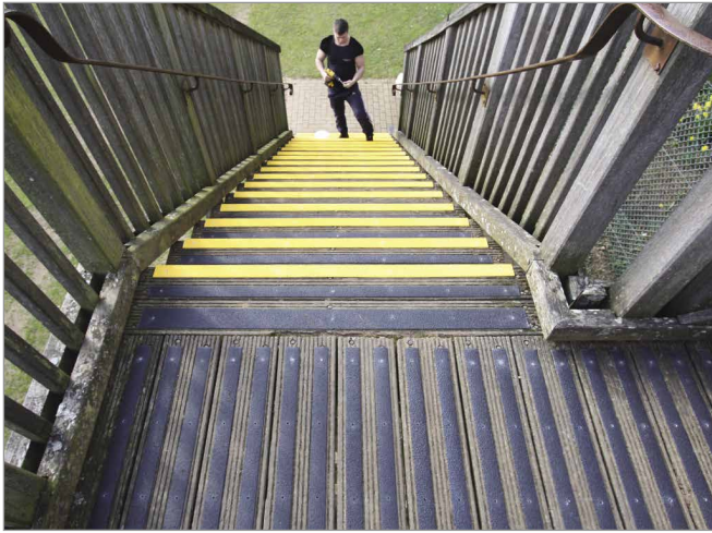
Public footbridge and stairs installation.
