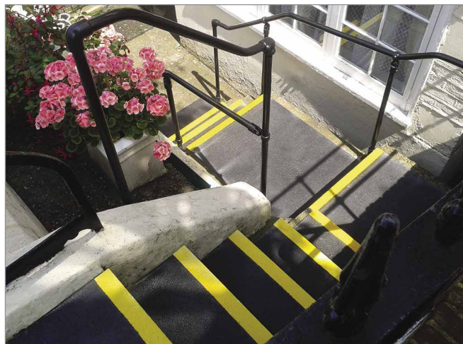
Use extra deep Stair Treads for landing areas.
